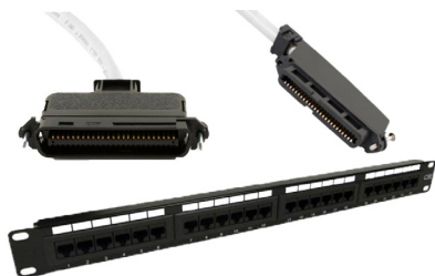
Paneles 19" 1U 24/25 puertos Telco RJ21 M 90°/0°
